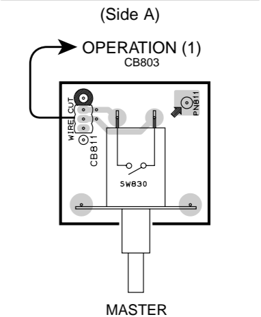
OPERATION (6) P.C.B. (Side A)
