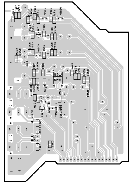
FUNCTION (4) P.C.B. (Side B) Lead Free Solder Used
